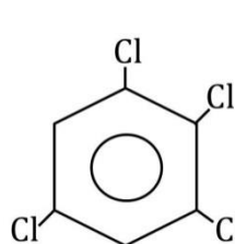
1,2,3,5-tetraclorobenceno
