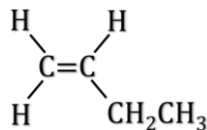
1-buteno
