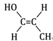
trans-1-propen-1-ol
