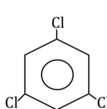
1,3,5-triclorobenceno
