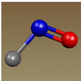
FNO: C_s
