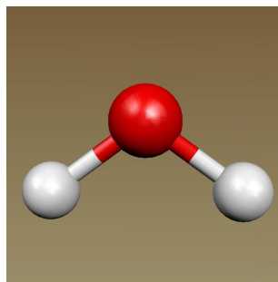
H 2 O: C_{2v}
