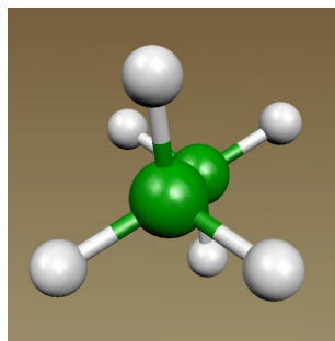
C 2 H 6 : D_{3d}
