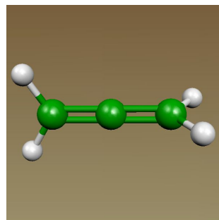
C 3 H 4 : D_{2d}
