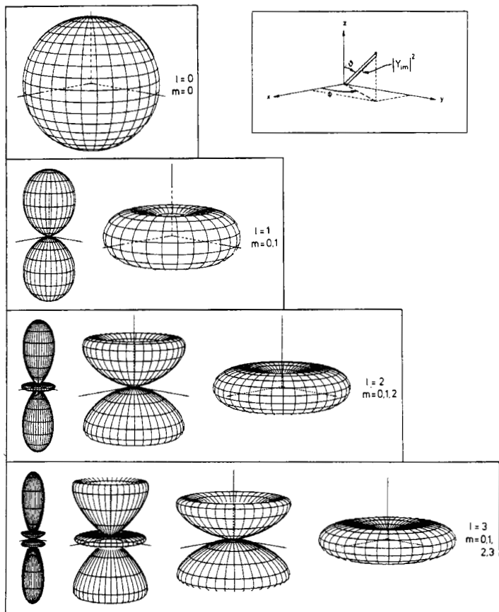
Figure 8.6: Polar diagrams of |Y_l^m(\theta)|^2 . The distance from the origin of the coordinate system to the point on the surface at angles \theta and \phi is equal to |Y_l^m(\theta)|^2 .
