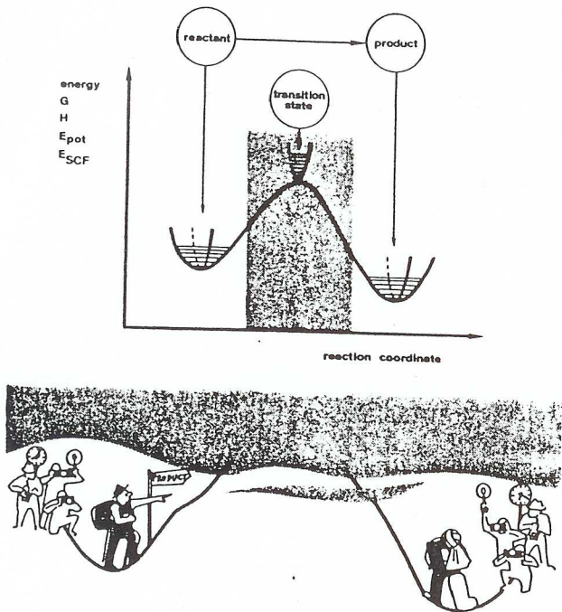
Fig. 1. Reaction energy profile for a one-step chemical transformation.
