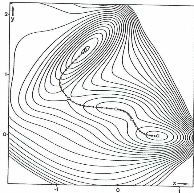
Fig. 15. Approximate minimum-energy reaction path for the two-parametric model potential by means of descending path points.
