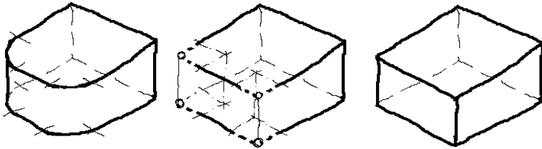
Fig. 2. Part with two rounds (left), arcs removed, edges extended and new vertices and edges added (middle), resulting polyhedral shape (right)
