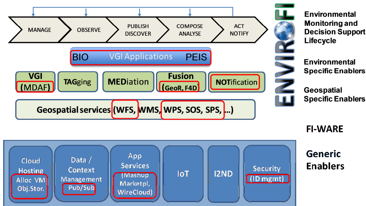
Figure 2 ENVIROFI architecture related to the VGI applications
