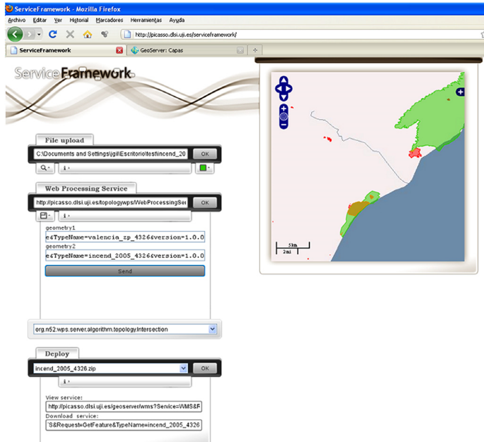
Fig. 6. Process results are deployed as standard services and visualized on the viewer.
