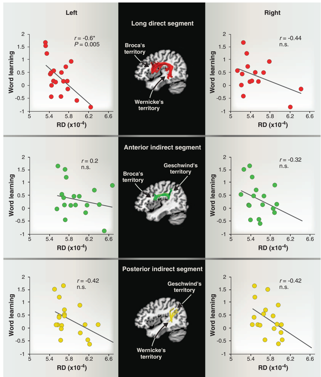
Fig. 4. Relation between individual ability to learn to segment new words from a speech stream and microstructure of the arcuate fasciculus. The latter is a fiber tract linking temporal cortex (Wernicke's territory) and inferior frontal cortex (Broca's territory), as well as premotor cortex. Each scatterplot represents individual word learning scores, expressed by d-prime measures, and the radial diffusivity (RD), a measure of white-matter structure. This anatomical feature is significantly predictive of word learning for the direct segment of the arcuate fasciculus (shown in red in top panel) in the left hemisphere. Indirect connections (middle and bottom panels) do not show a significant relationship. [Adapted with permission from (56)]
